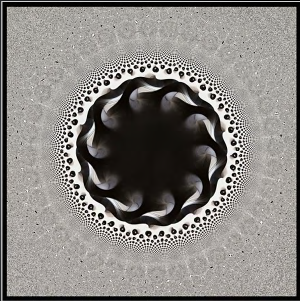
Black Hole
